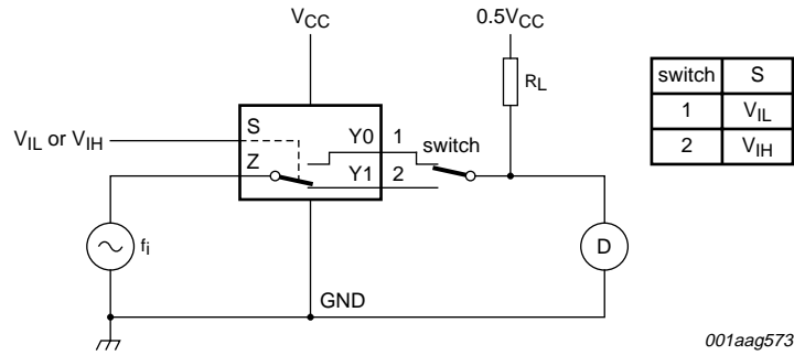
Fig 16. Test circuit for measuring total harmonic distortion
