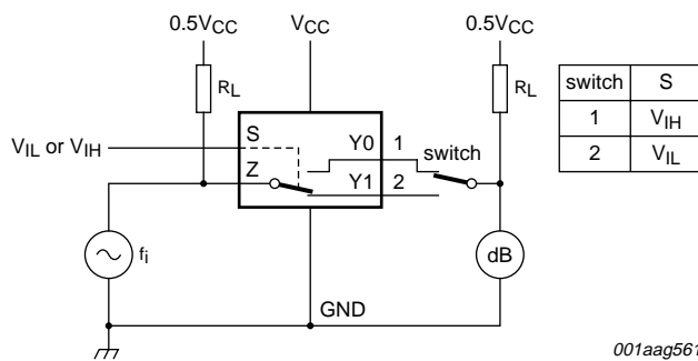
Fig 18. Test circuit for measuring isolation (OFF-state)
