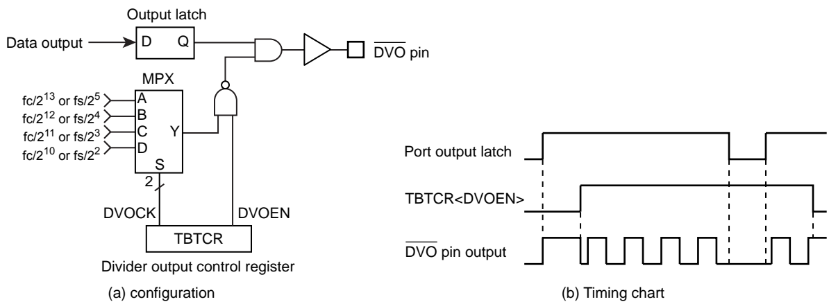
Figure 7-3 Divider Output
