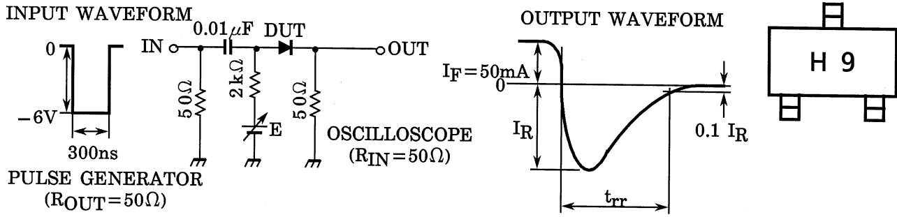
Fig.1 Reverse Recovery Time ( t_{rr} ) Test Circuit Marking
