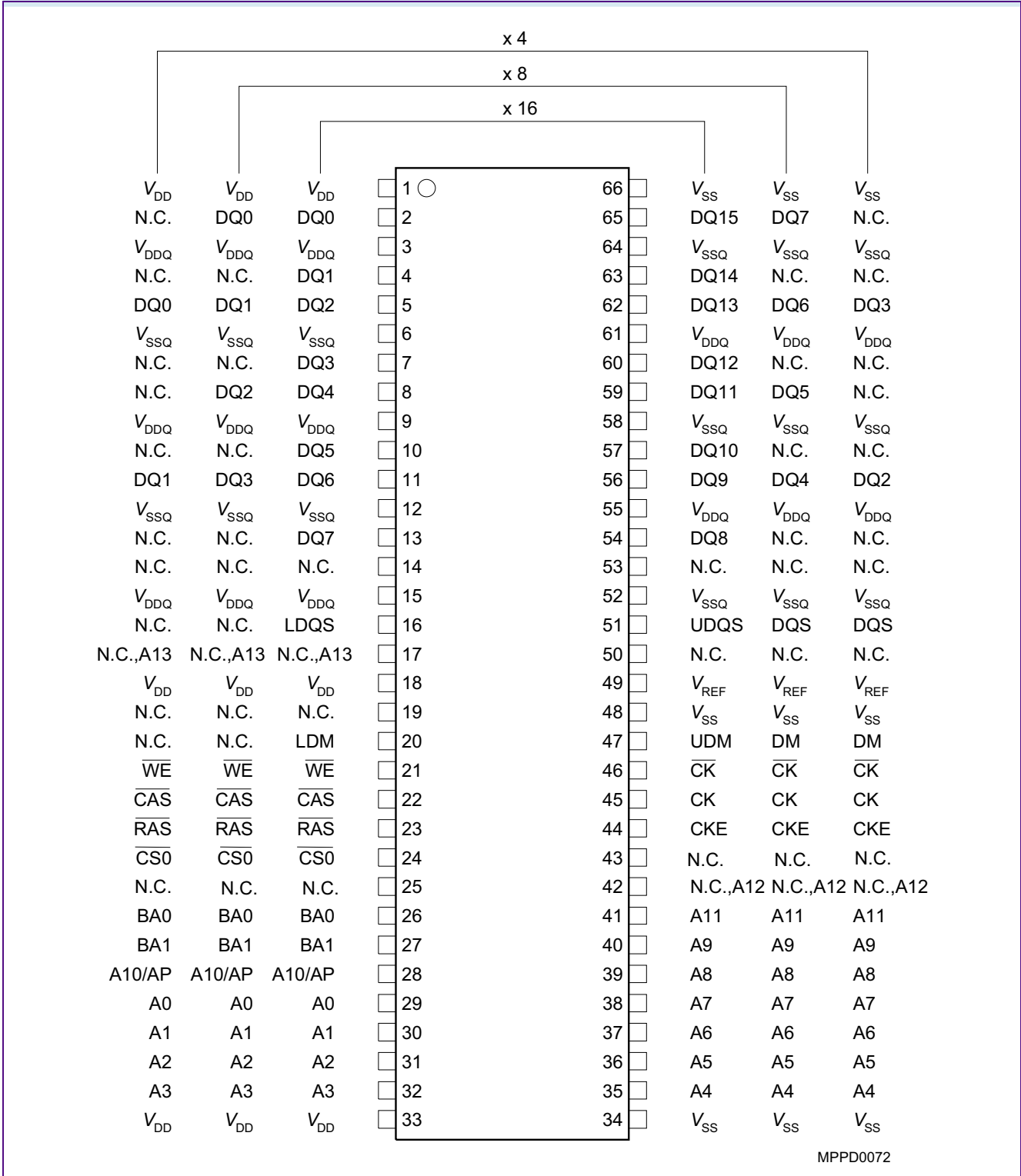
FIGURE 2 Pin Configuration P(G)-TSOPII-66
