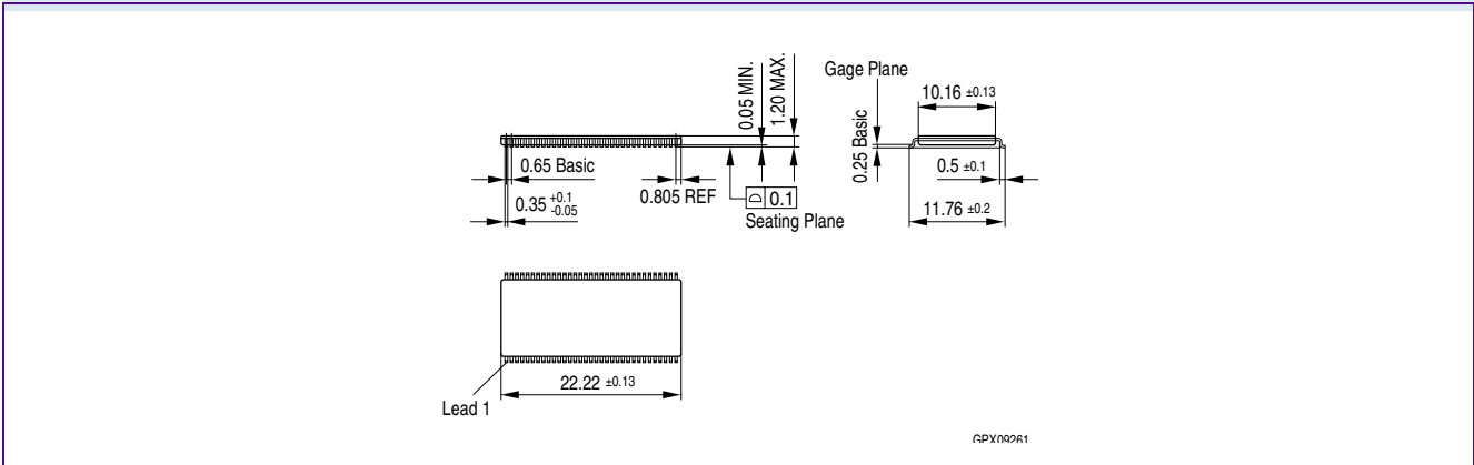
FIGURE 5 Package Outline of P(G)-TSOPII-66-1 (green/non-green)
