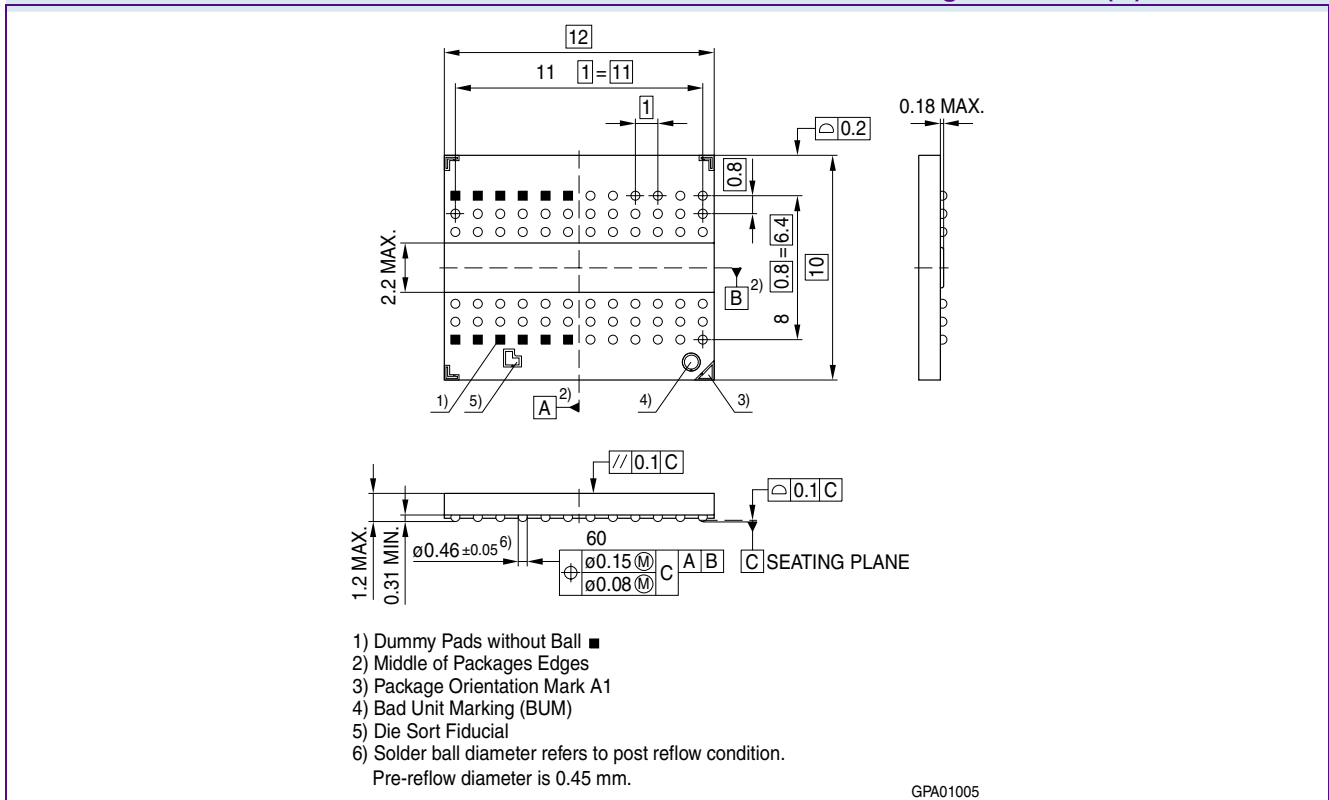
Package Outline P(G)-TFBGA-60-11
