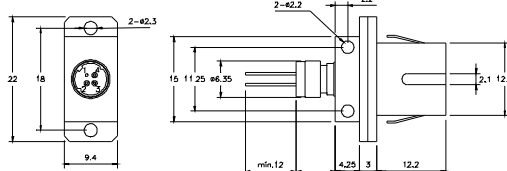
SC Receptacle (Board Mount)
