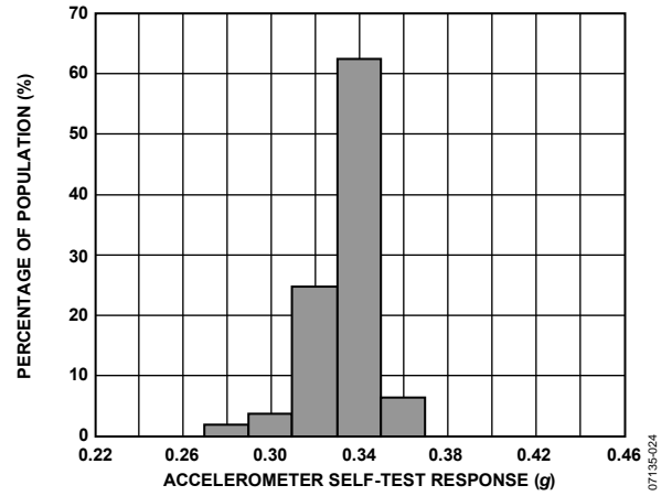
Figure 25. Accelerometer Self-Test Distribution, 25°C
