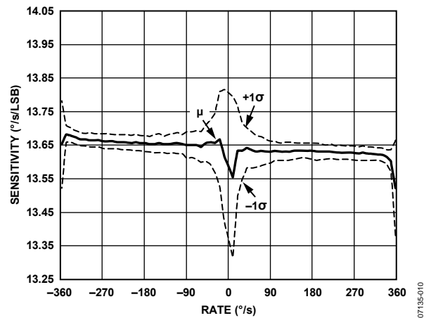
Figure 11. Gyroscope Linearity
