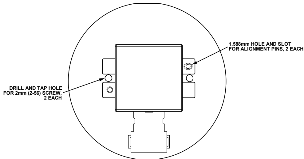
Figure 31. Mechanical Attachment
