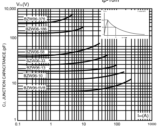
FIG.4- CLAMPING VOLTAGE VERSUS PEAK PULSE CURRENT. EXPONENTIAL WAVEFORM tp=200μs, tp=1ms, tp=10m
