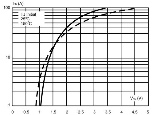
FIG.7- PEAK FORWARD VOLTAGE DROP VERSUS PEAK FORWARD CURRENT (TYPICAL VALUES FOR UNIDIRECTIONAL TYPES)
