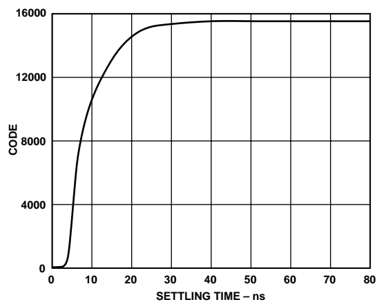
Figure 23. Settling Time
