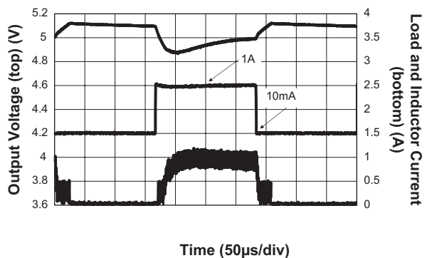
Load Transient ( V_{OUT} = 5V; C_{FF} = 100pF )
