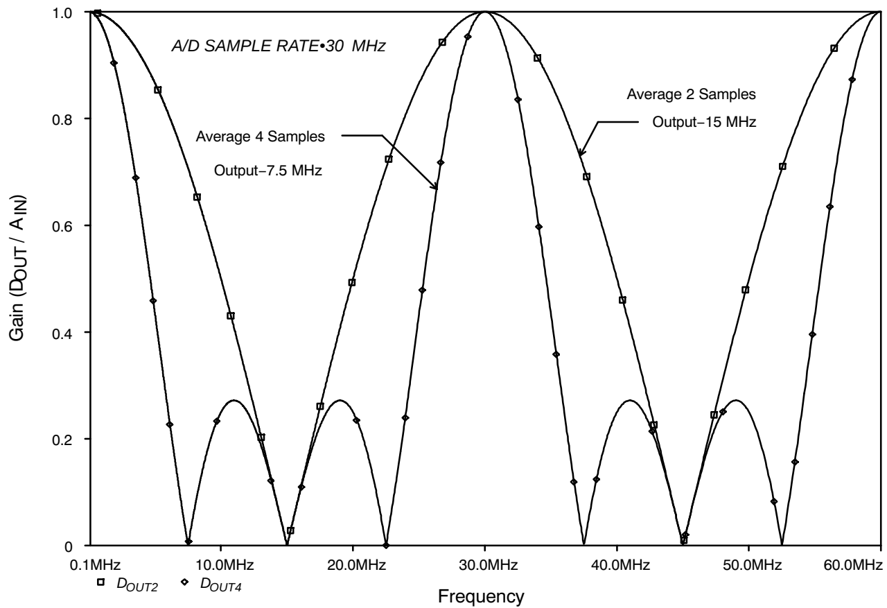
Graph 1. Decimation Filter Frequency Response
