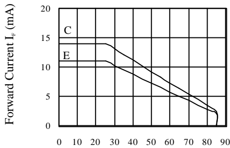
FIG.3 ALLOWABLE DC CURRENT VS. AMBIENT TEMPERATURE
