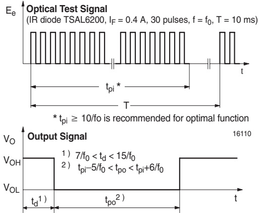
Figure 1. Output Function
