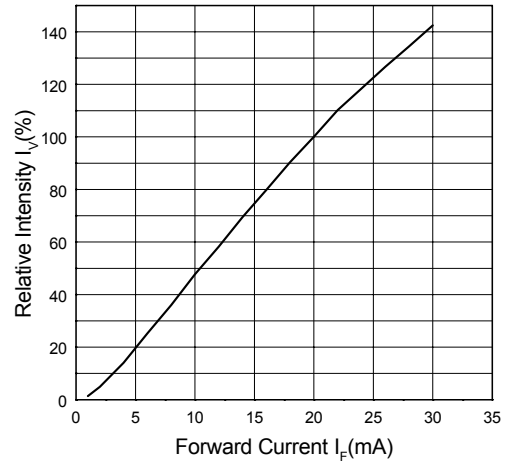
Relative Intensity I_v (%) vs Forward Current I_F (mA)
