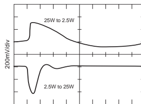
25W to 2.5W 2.5W to 25W 50 \mu s/div 10% \leftrightarrow 100% SMTR2805S STEP LOAD RESPONSE
