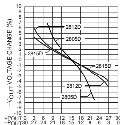
-VOUT VOLTAGE CHANGE (%) OUTPUT LOAD (Watts) 10% to 90% LOAD +V 90% to 10% LOAD -V CROSS REGULATION FIGURE 19
