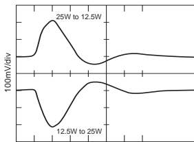
25W to 12.5W 12.5W to 25W 50 \mu s/div 50% \leftrightarrow 100% SMTR2805S STEP LOAD RESPONSE
