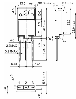
TO-3PM
