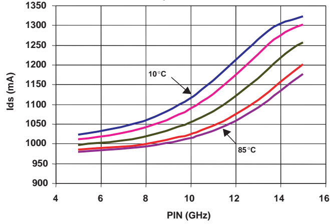
RMPA39100 Power, I_{ds} vs. Temperature Frequency = 39 GHz, Bias V_d = 5V , I_d = 1000mA Base Plate Temp 10, 25, 50, 75, and 85°C
