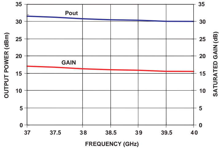
RMPA39100 Saturated Power and Gain vs. Frequency P_{in} = 14.5 \text{ dBm} , Bias V_d = 5V , I_d = 1000mA , T = 25^\circ\text{C}
