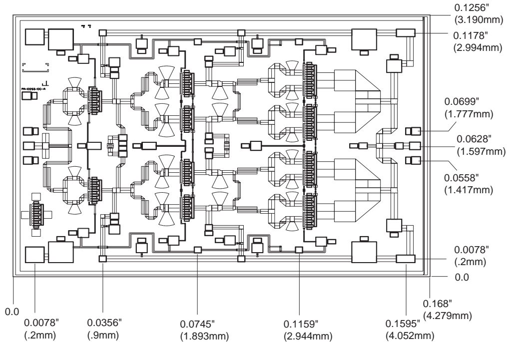
Figure 2. Chip Layout and Bond Pad Locations (Chip Size is 4.28mm x 3.19mm x 50µm. Back of chip is RF and DC Ground)
