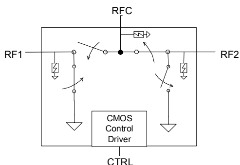
Figure 1. Functional Schematic Diagram
