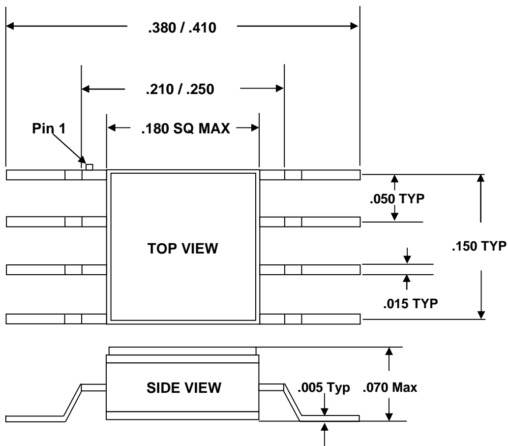
Figure 14. Package Drawing
