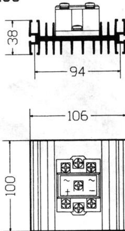
1. Application example using a SEMIPONT bridge module and heatsink P 5A/100 to give single phase bridge rectifier
