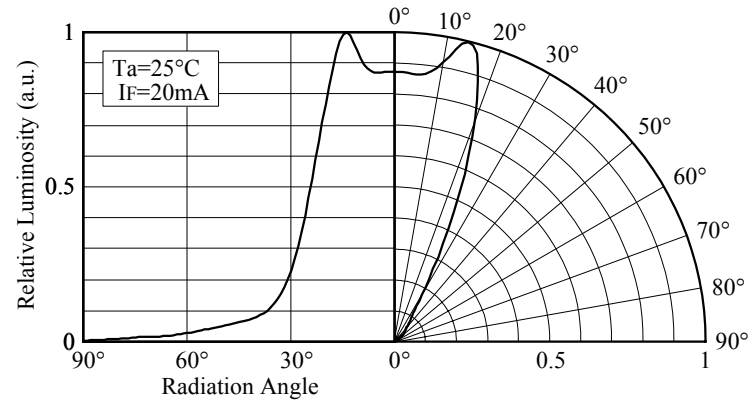
■ Directivity (NSPW510B(S))
