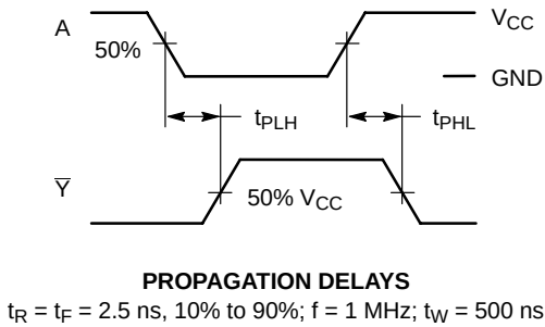
Figure 3. Switching Waveforms
