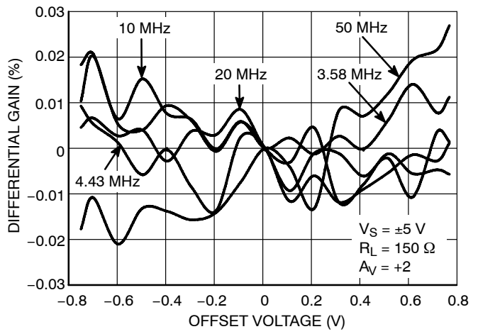
Figure 16. Differential Gain
