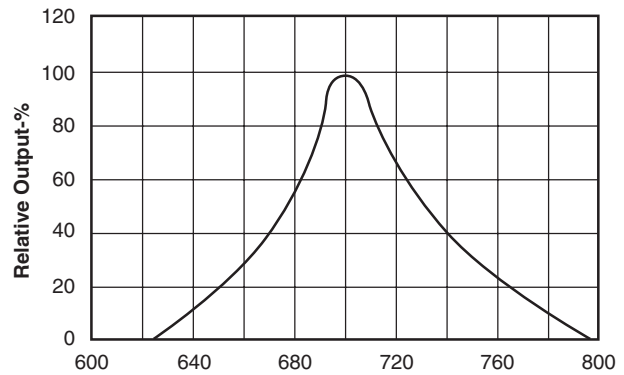
Fig. 2 Spectral Response
