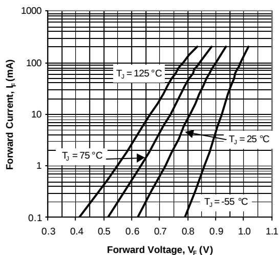
Figure 2. Forward Voltage
