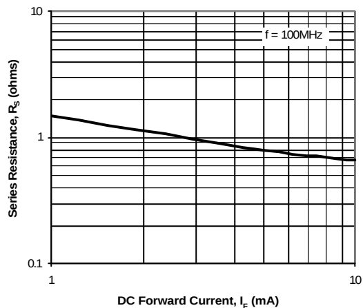
Figure 4. Series Resistance
