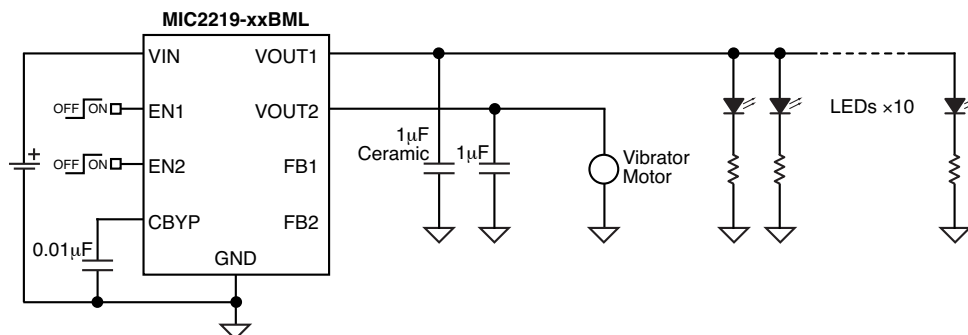
MIC2219 Typical Cell Phone Application
