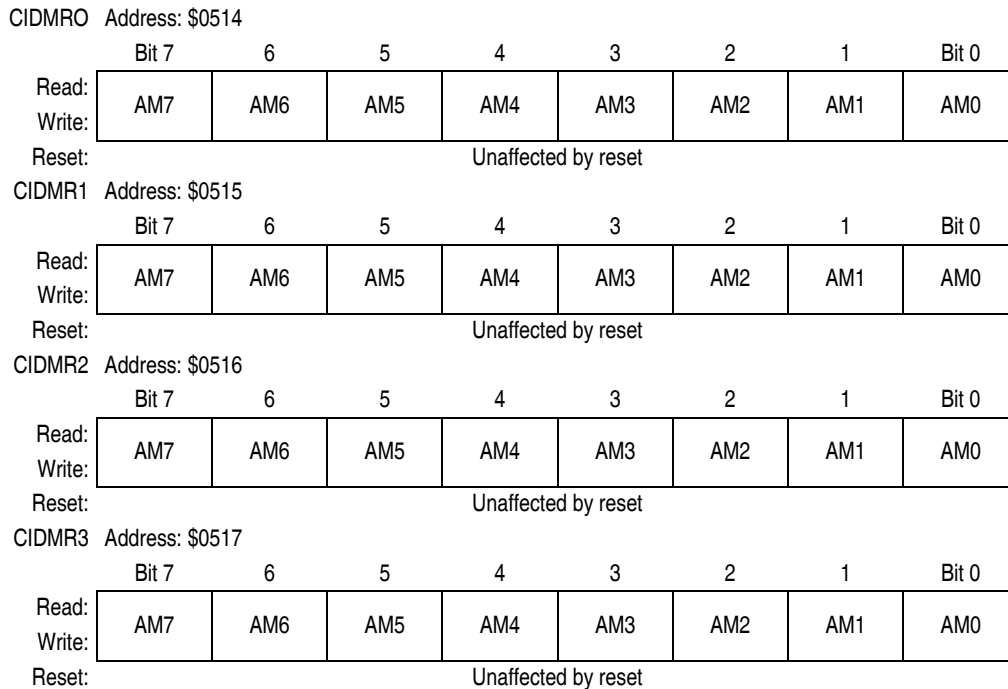
Figure 12-28. Identifier Mask Registers (CIDMR0–CIDMR3)
