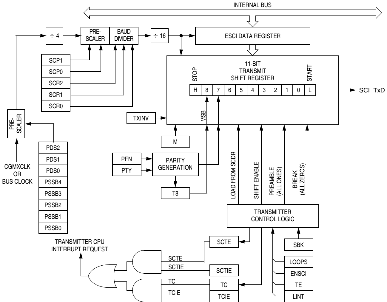
Figure 14-5. ESCI Transmitter
