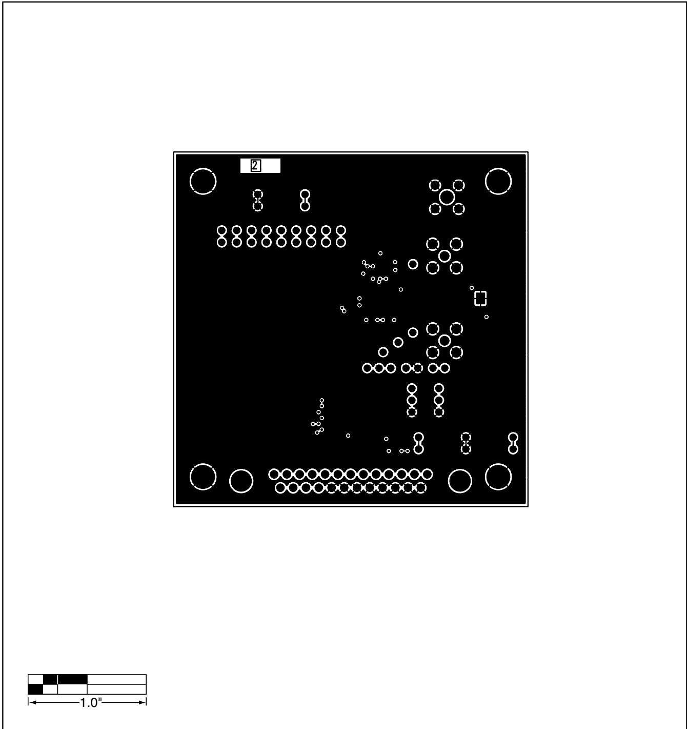
Figure 4. MAX2160 EV Kit PC Board Layout—Inner Layer 2
