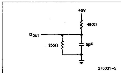
Load B
