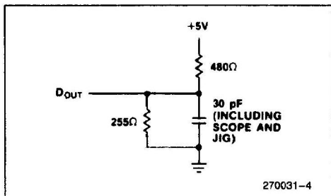
Load A
