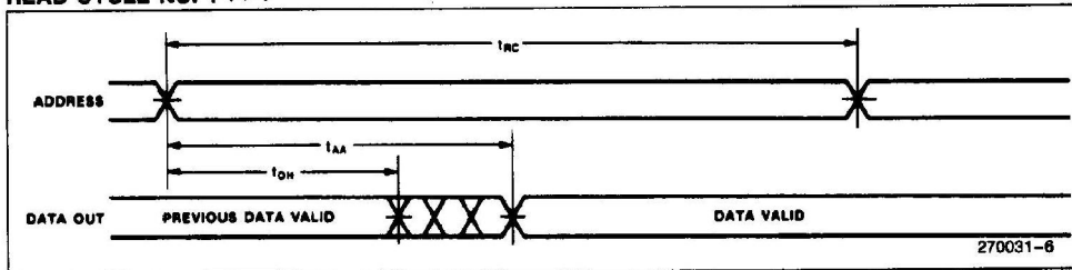
READ CYCLE NO. 1 (1, 2)
