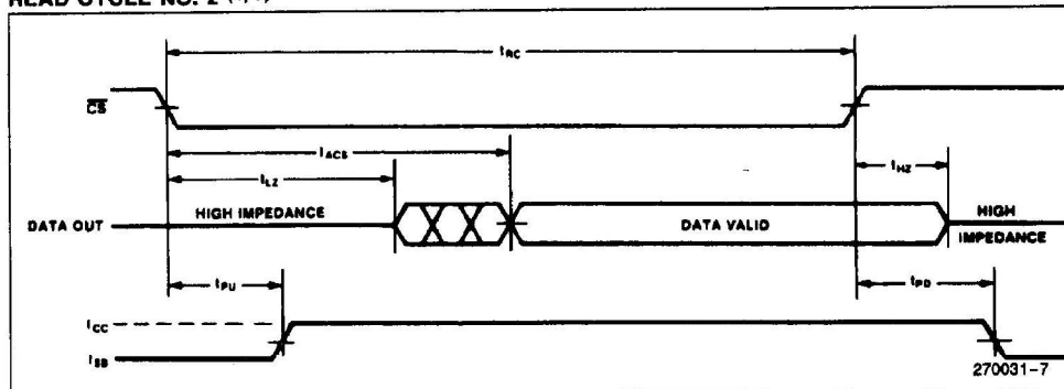
READ CYCLE NO. 2 (1, 3)
