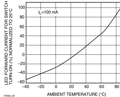
Figure 4. LED Current for Switch Turn-on vs. Temperature
