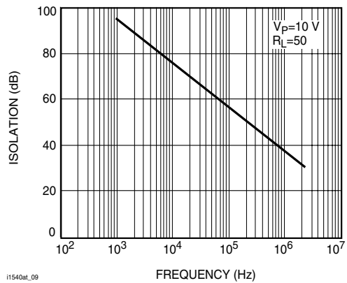
Figure 10. Output Isolation
