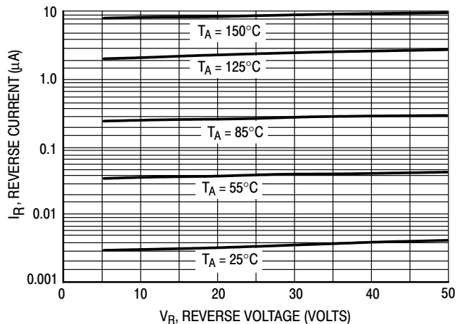
Figure 4. Leakage Current
