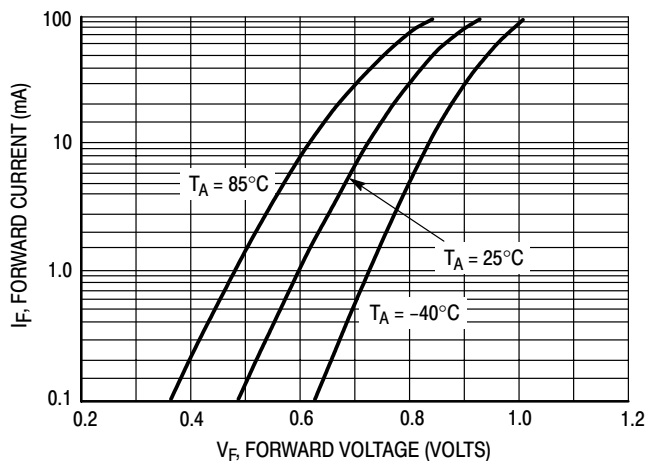
Figure 3. Forward Voltage
