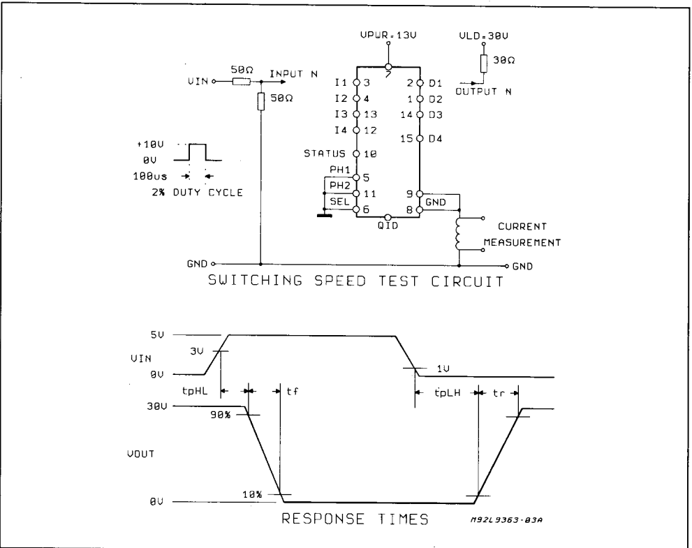
Figure 1: Response Times.
