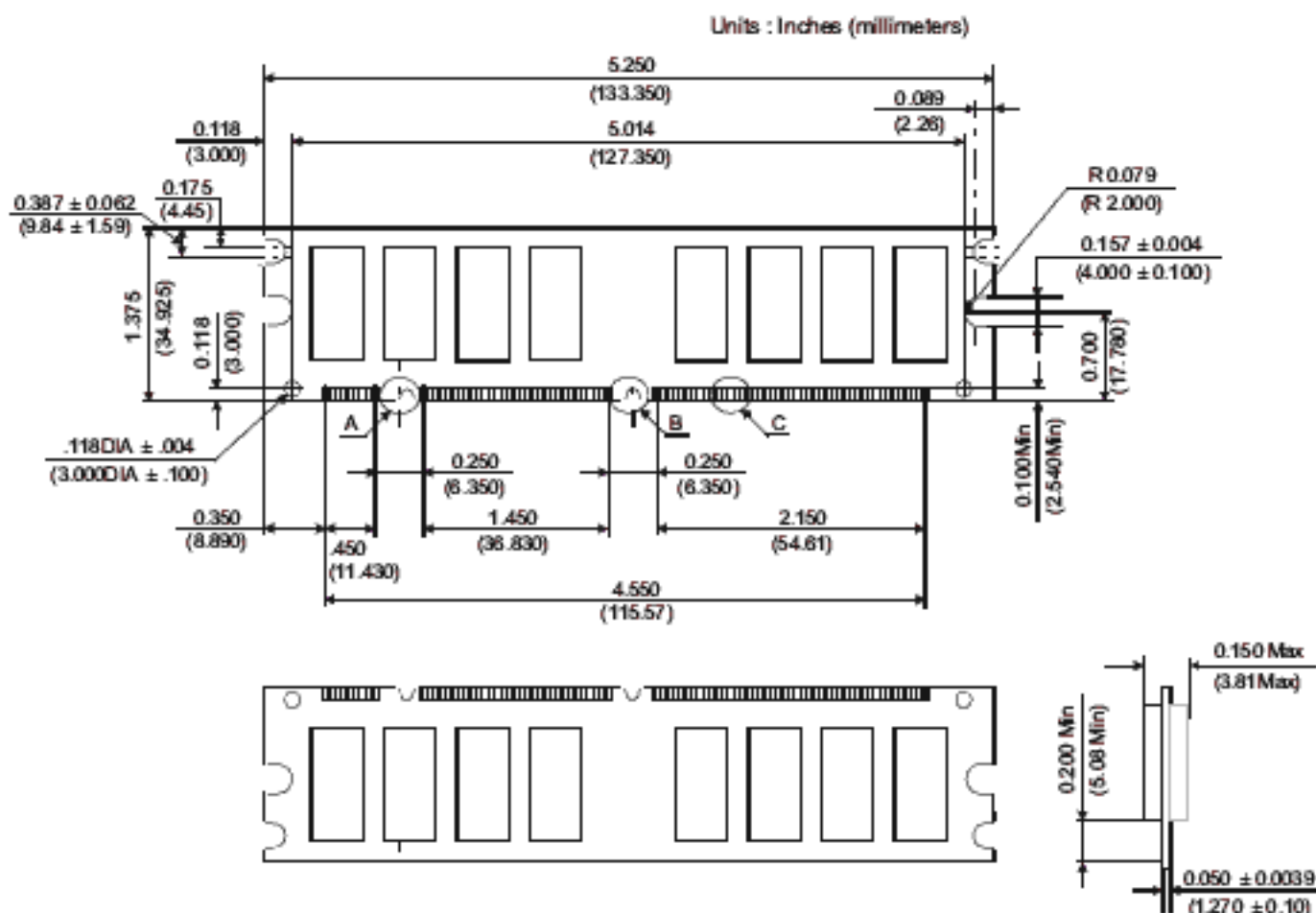
Figure 1: KVR133X64C3/512 168-Pin SDRAM Module
