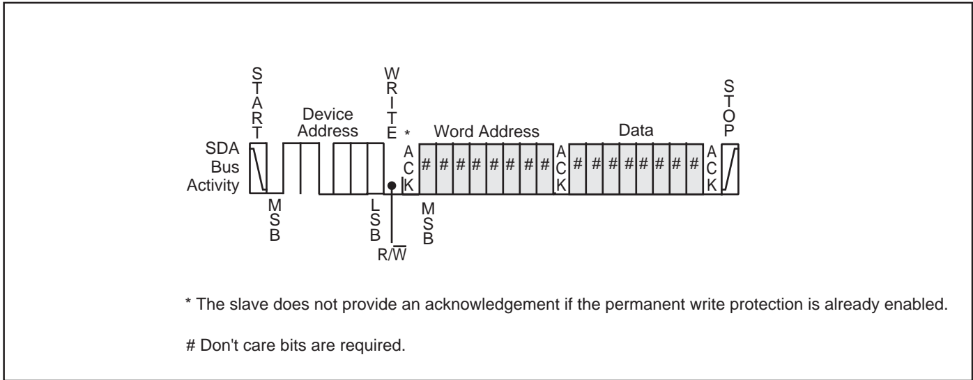
FIGURE 11. PERMANENT WRITE PROTECTION INITIATION
