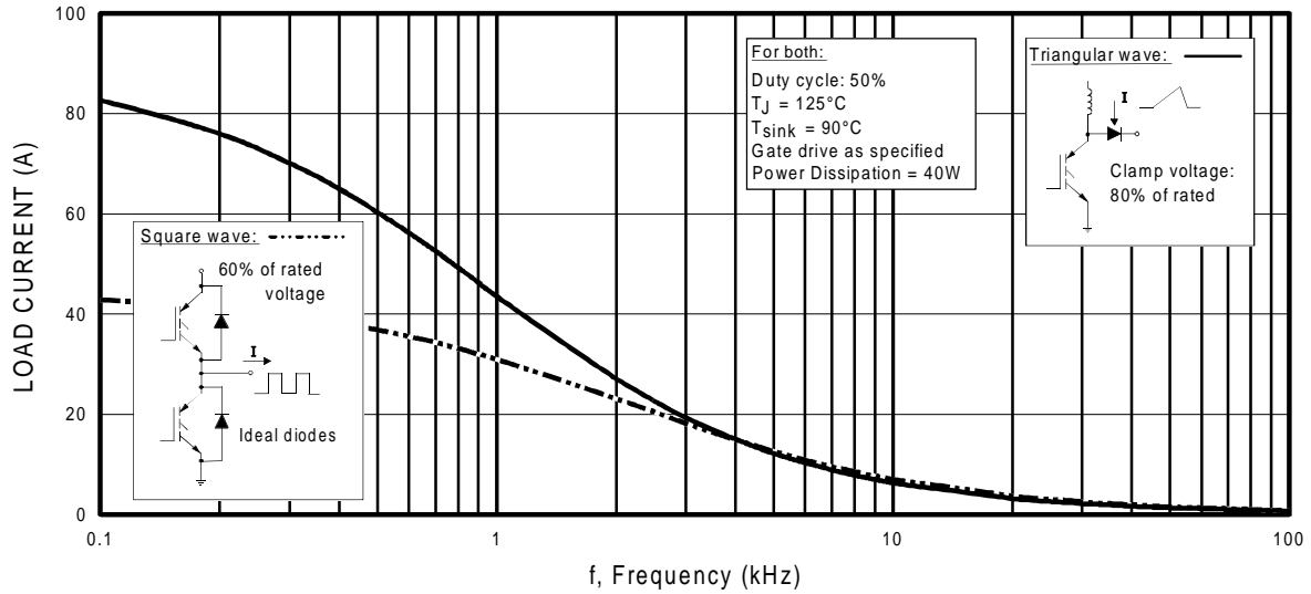
Fig. 1 - Typical Load Current vs. Frequency (For square wave, I = I_{RMS} of fundamental; for triangular wave, I = I_K )
