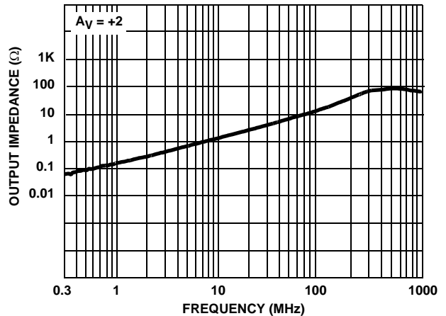
FIGURE 20. OUTPUT IMPEDANCE
