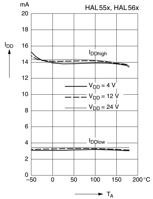
Fig. 3-6: Typical current consumption versus ambient temperature
