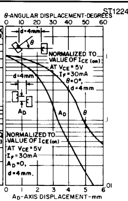
Fig 6B. Output Current vs. Displacement (Angular & Axis)
