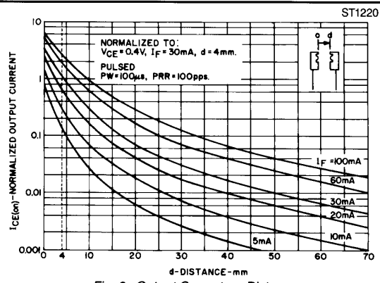
Fig. 3. Output Current vs. Distance
