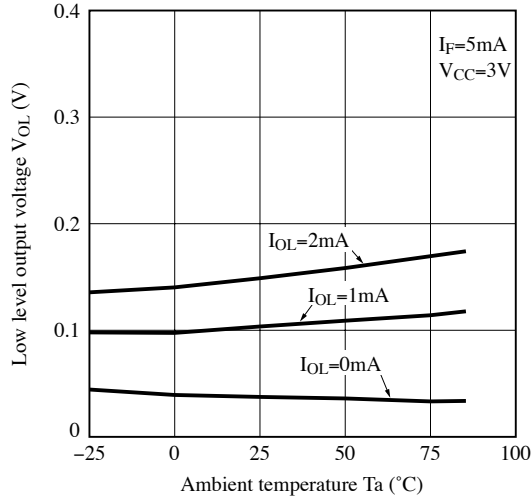
Fig.12 Low Level Output Voltage vs. Ambient Temperature
