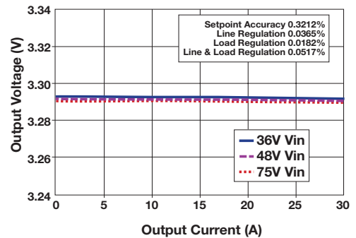
Line/Load Regulation
