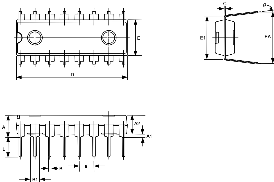
DIP-16L Package
