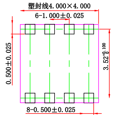
LAND PATTERN RECOMMENDATION 推荐焊盘图
