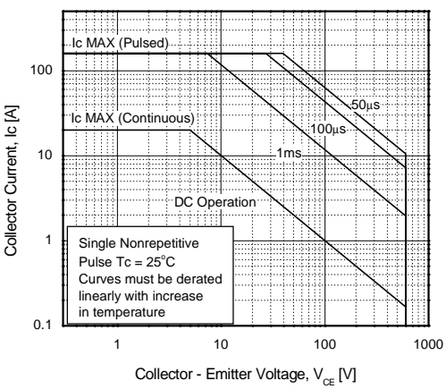
Fig 15. SOA Characteristics
