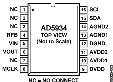
Figure 3. Pin Configuration
