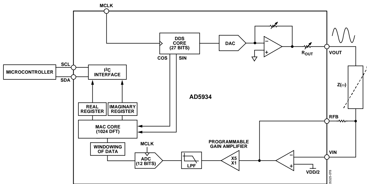
Figure 14. AD5934 Block Overview
