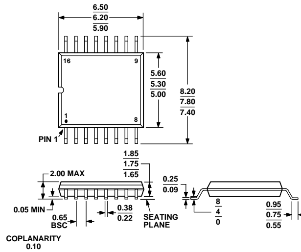
Figure 37. 16-Lead Shrink Small Outline Package [SSOP] (RS-16) Dimensions shown in millimeters
