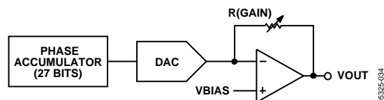
Figure 16. AD5934 Transmit Stage
