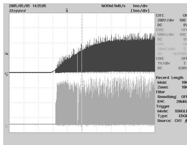
Figure 15 – 264 VAC Input and Maximum Load. Lower: I_{DRAIN} , 0.2 A / div. Upper: V_{DRAIN} , 200 V & 1 ms / div.
