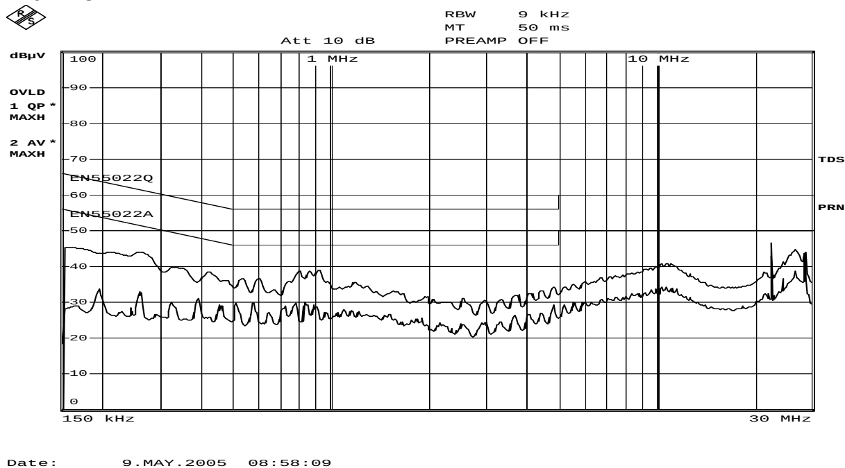
Figure 25 – Conducted EMI, Maximum Steady State Load, 230 VAC, 60 Hz, and EN55022 B Limits
