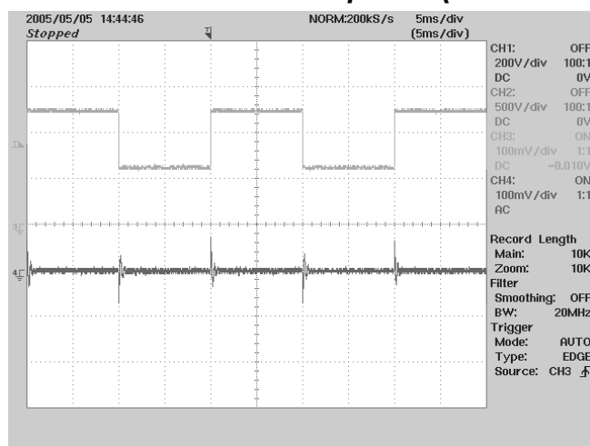
Figure 16 – Transient Response, 90 VAC, 50-100-50% Load Step. Upper: Load Current, 1 A/div. Lower: Output Voltage 100 mV/ div, 5 ms / div.
