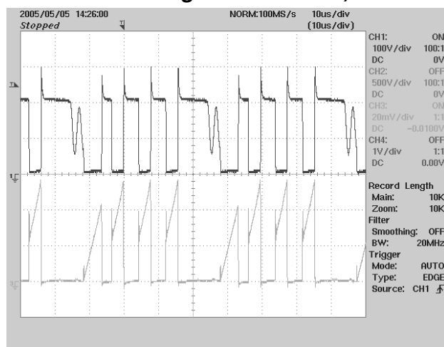
Figure 10 – 90 VAC, Full Load.
