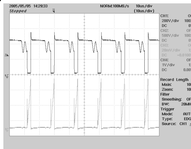
Figure 11 – 264 VAC, Full Load
