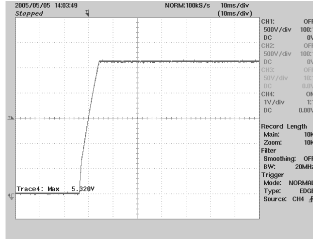
Figure 13 – Start-up Profile, 264 VAC, Full load 1 V / div, 10 ms / div.
