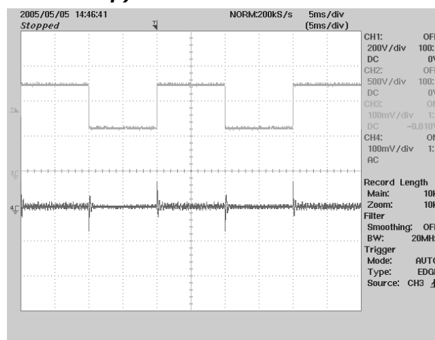
Figure 17 – Transient Response, 264 VAC, 50-100-50% Load Step Upper: Load Current, 1 A/ div. Lower: Output Voltage 100 mV/ div, 5 ms / div.
