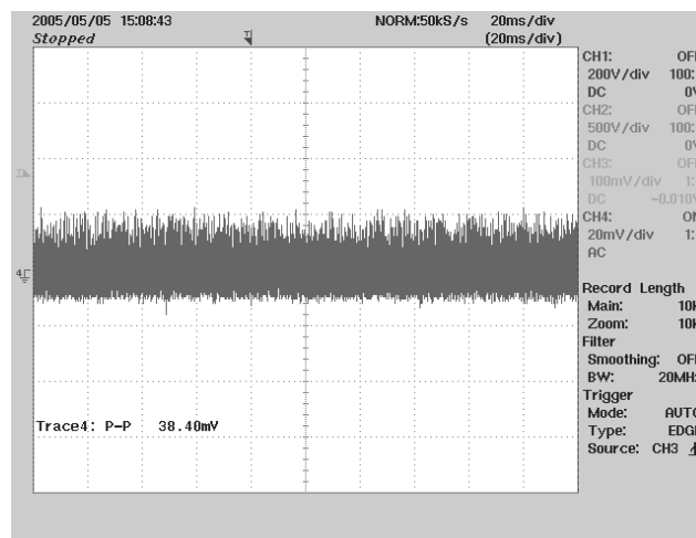
Figure 23 – 5.25V Ripple, 264 VAC, Full Load. 20 ms/ div, 20 mV / div
