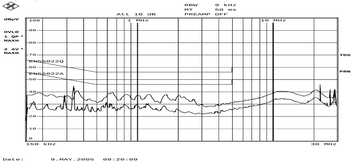
Figure 24 – Conducted EMI, Maximum Steady State Load, 115 VAC, 60 Hz, and EN55022 B Limits
