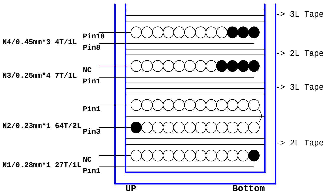
Figure 5 – Transformer Build Diagram.
