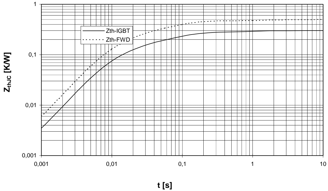
Transienter Wärmewiderstand Wechsell. Z_{thJC} = f(t) Transient thermal impedance Inverter
