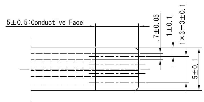
Conductive Face FPC-Type Cable
