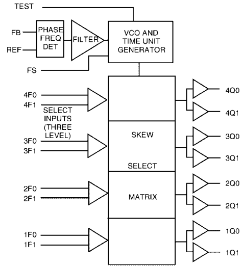
Logic Diagram
