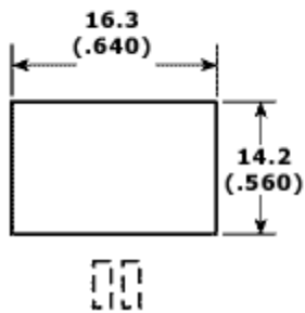
Recommended Cu Heat Spreader Drain Pad
