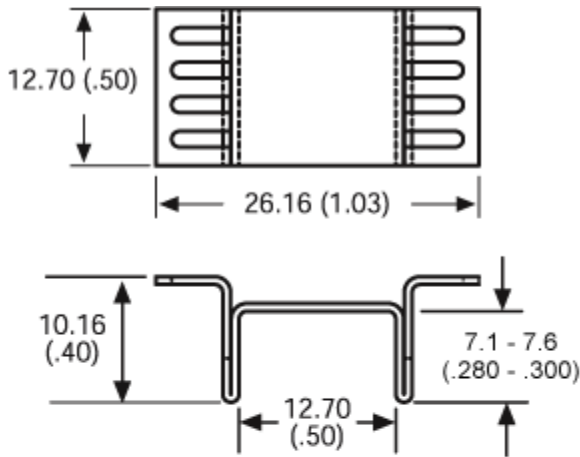
Recommended Cu Heat Spreader Drain Pad
