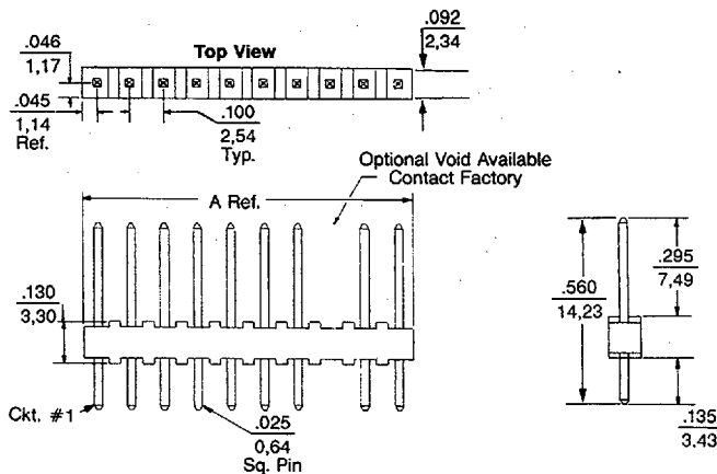
Recommended P.C. Board Layout for .100" (2.54 mm) Headers
