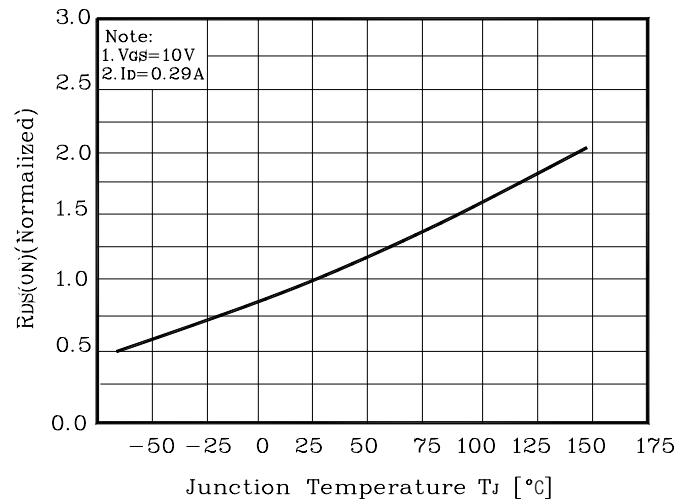
Fig. 8 R_{DS(on)} - T_J
