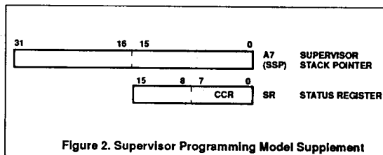
Figure 2. Supervisor Programming Model Supplement
