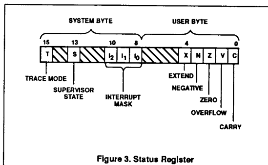
Figure 3. Status Register
