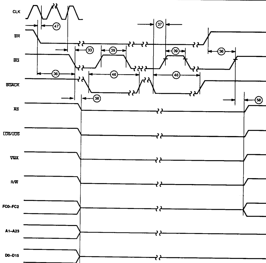
Figure 52. Bus Arbitration Timing Diagram — Multiple Bus Requests
