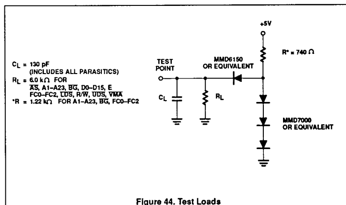
Figure 44. Test Loads
