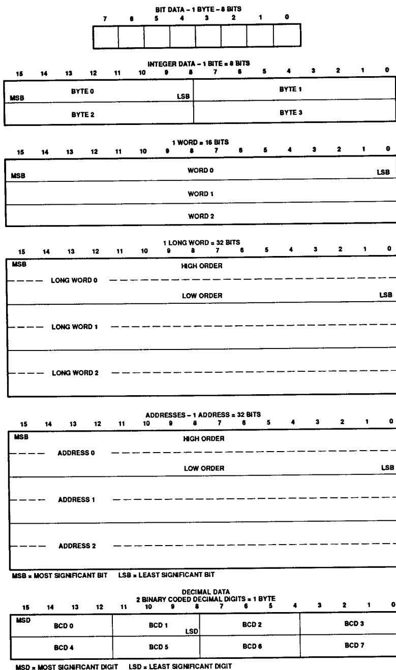
Figure 5. Memory Data Organization
